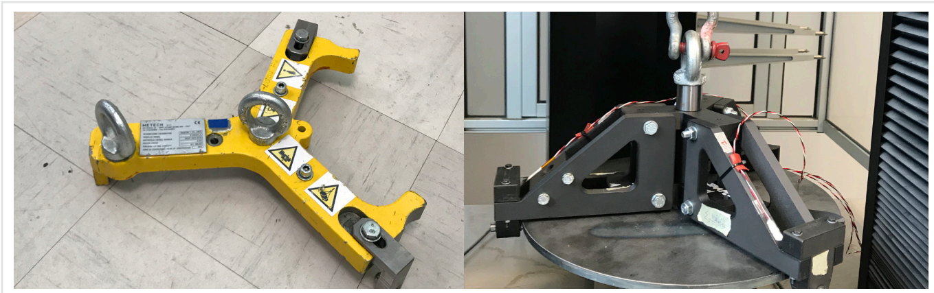
The original lifting tool (L) was machined out of solid steel and weighed 75% more than its 3D printed replacement (R).
