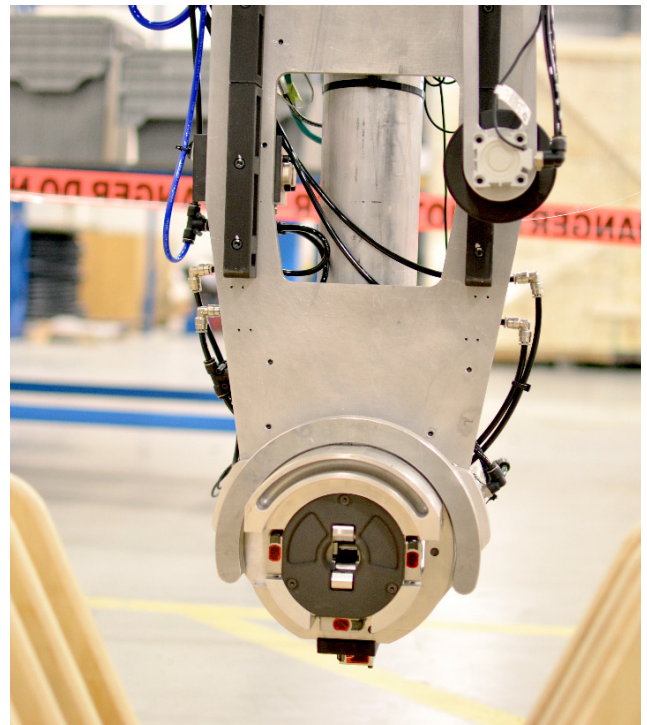
Several of the 3D printed parts were reinforced with Kevlar®, HSH fiberglass, and carbon fiber
